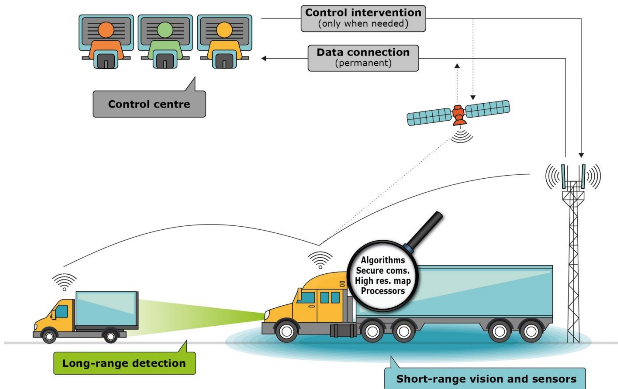
Figure 2. Stylised driverless truck operating environment (with optional Control Centre)
